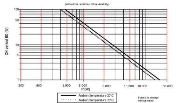
Pulse carrying capacity, brake resistor
